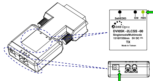
Figure 1 The LEDs denoted by arrows will be turned on in transmitter
